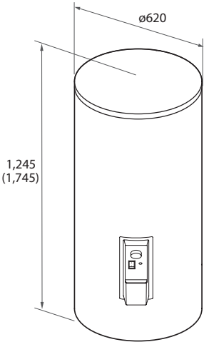
REW-SA200S/REW-SA300S
