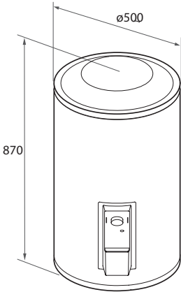
REW-SA100S
