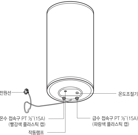
REW-SA100W
