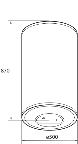
REW-SA100W
