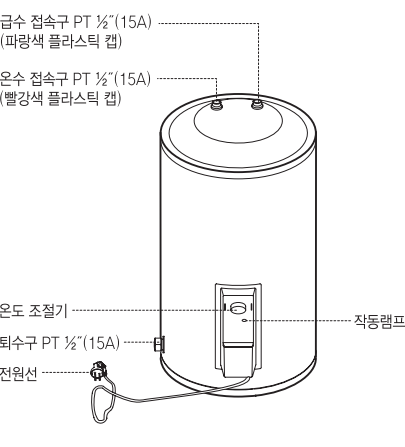
REW-SA100S
